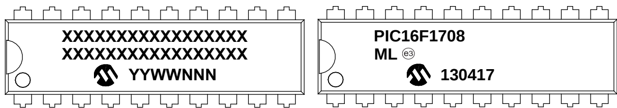
20-Lead PDIP (300 mil)
