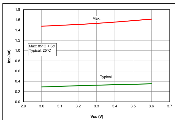
FIGURE 33-41: I_{DD} , Low-Power Brown-out Reset, LPBOR = 0 . PIC16LF1704/8 Only.
