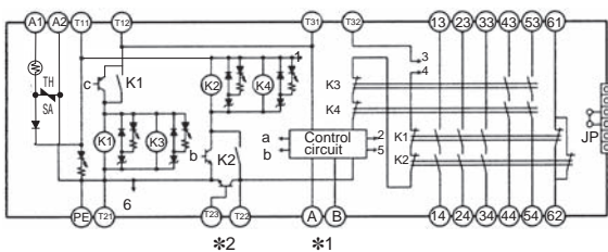
G9SA-321-T□ (24 VAC/VDC)
