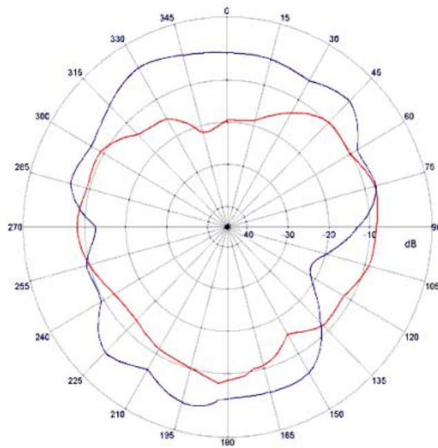
Figure 21 – Y-Z Plane Antenna Pattern
