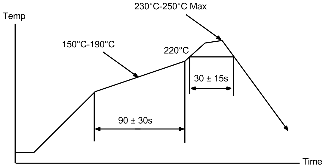
Figure 23 – Reflow Profile for Lead Free Solder
