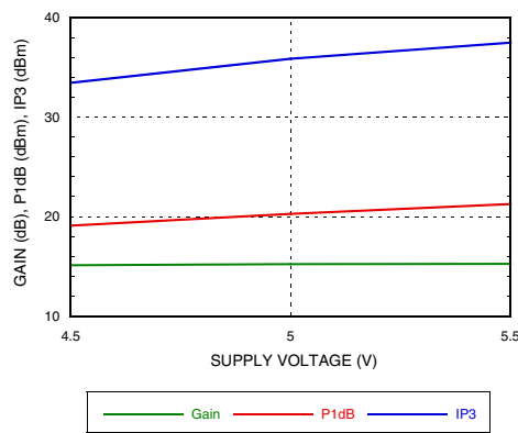
Gain & Power vs. Supply Voltage @ 1 GHz
