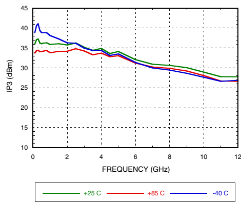
Output IP3 vs. Temperature [1]
