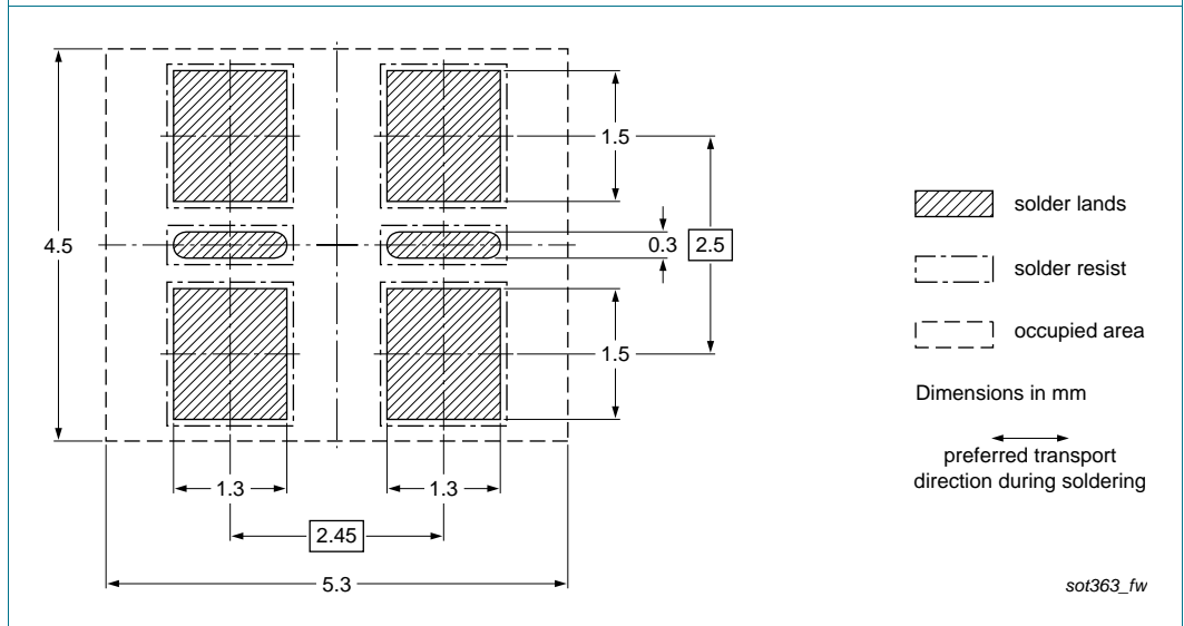
Fig 20. Wave soldering footprint PUMD15 (SOT363)
