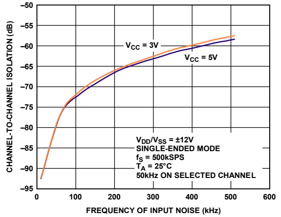
Figure 14. Channel-to-Channel Isolation
