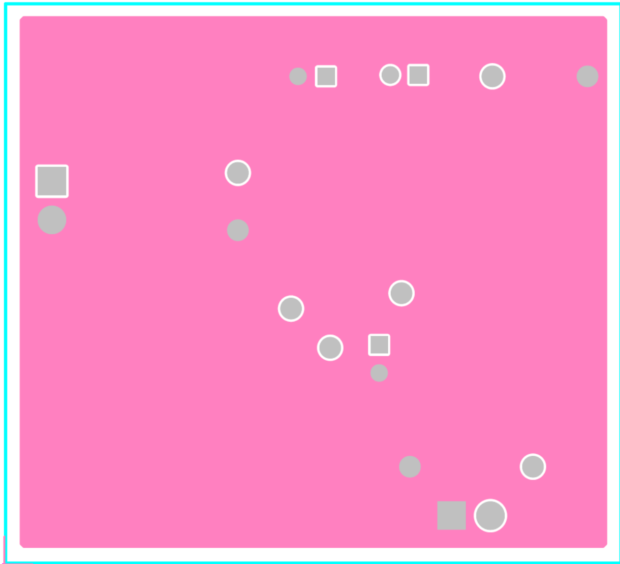
Figure 20. TPS54678EVM-155 Layout 2
