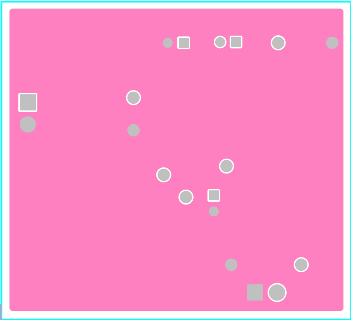
Figure 20. TPS54678EVM-155 Layout 2
