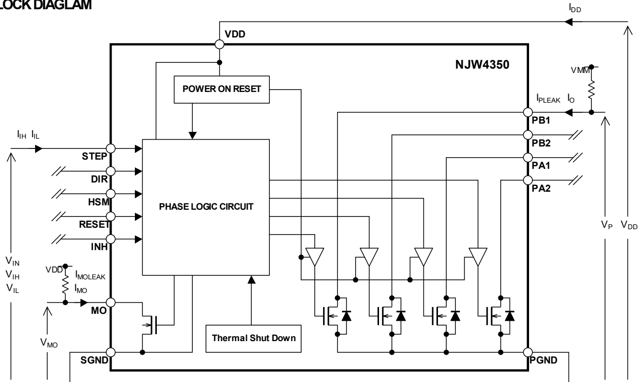
Fig.2 Block Diagram
