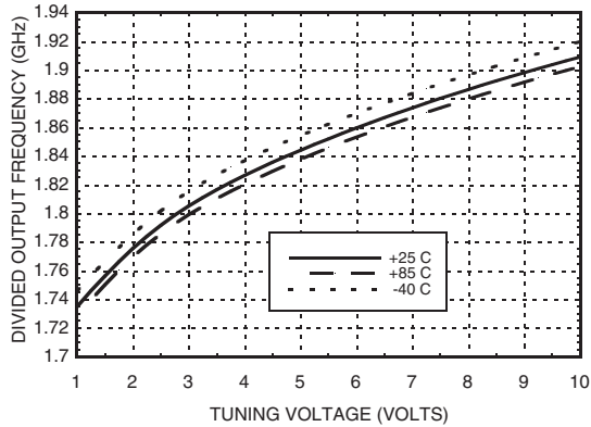
Divided Output Frequency vs. Tuning Voltage, Vcc= +5V
