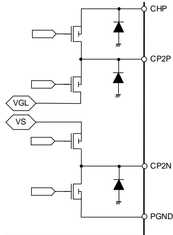
TYPE11: CHP, CP2P, CP2N, PGND
