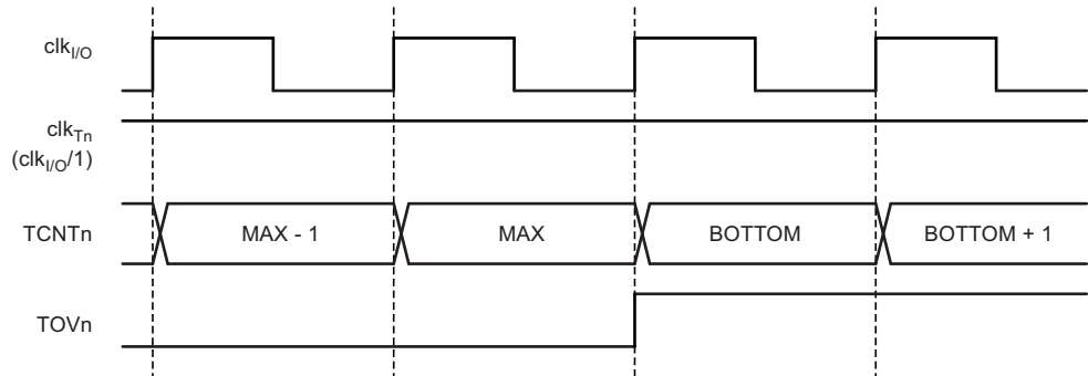
Figure 14-5. Timer/Counter Timing Diagram, no Prescaling
