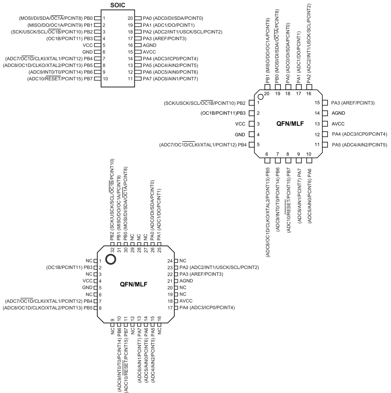
Figure 1-1. Pinout ATtiny261/461/861
