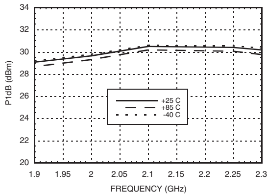
PIdB vs. Temperature @ 2100 MHz
