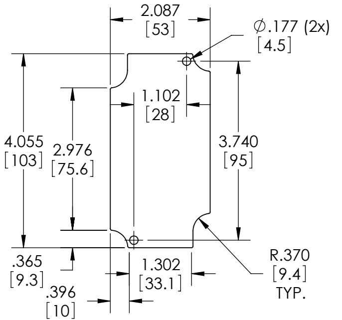
SUGGESTED PC BOARD LAYOUT
