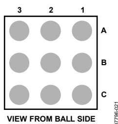
Figure 3. Pin Configuration
