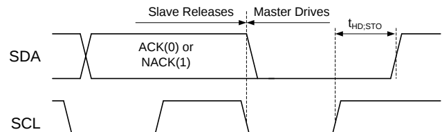
Figure 40. Stop Bit
