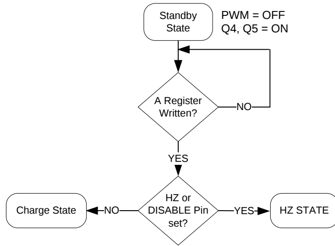
Figure 36. Standby State
