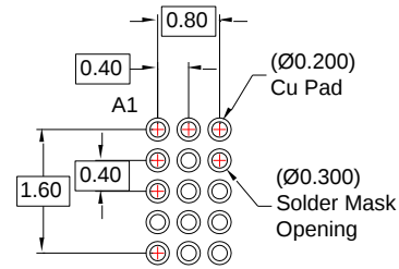
RECOMMENDED LAND PATTERN (NSMD TYPE)
