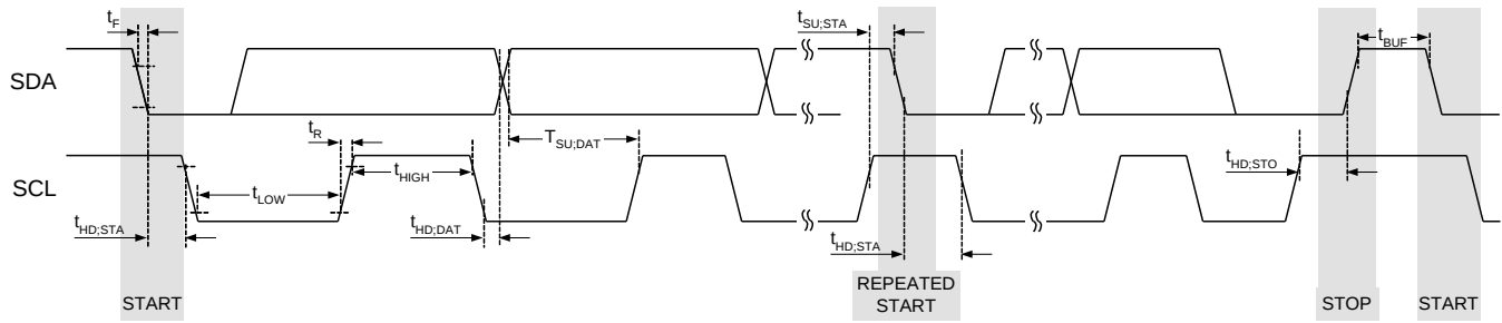
Figure 4. I²C Interface Timing for Fast Plus, Fast, and Slow Modes
