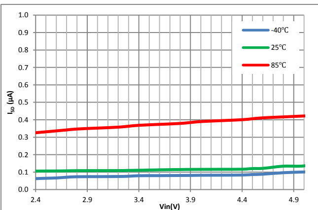
Figure 13. Shutdown Current vs. Input Voltage and Temperature
