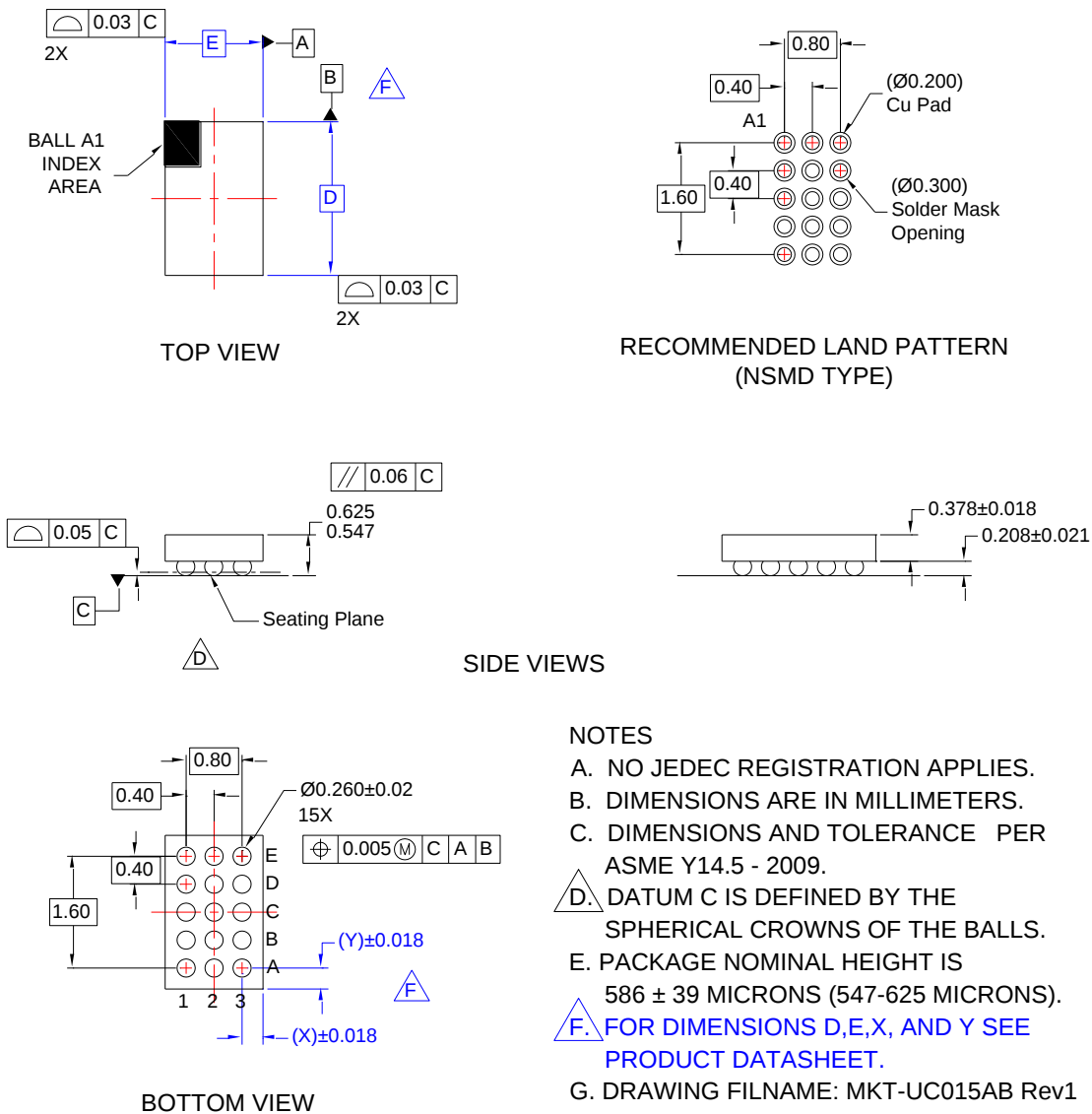
Figure 30. 15-Ball, Wafer-Level Chip-Scale Package (WLCSP), 3x5 Array, 0.4 mm Pitch, 250 µm Ball
