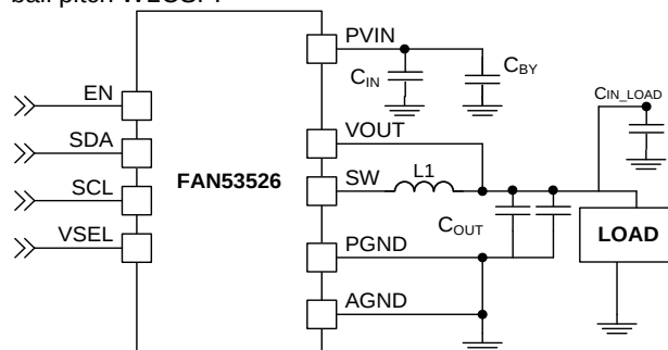
Figure 1. Typical Application
