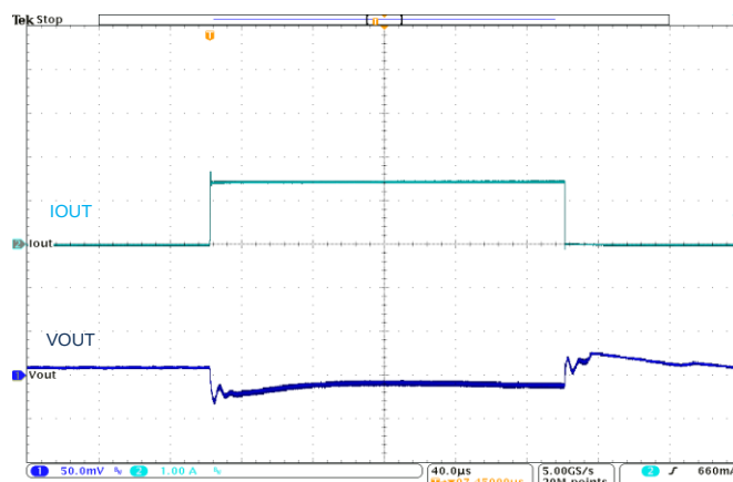
Figure 15. Load Transient, 3.6 V_{IN} , 1.15625 V_{OUT} , 0.01-1.5 A, 120 ns Edge
