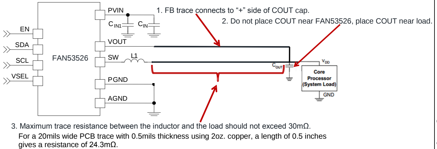
Figure 29. Remote Sensing Schematic
