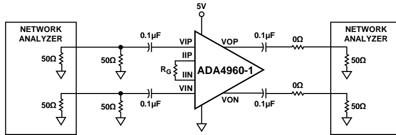
Figure 29. S-Parameter Test Circuit
