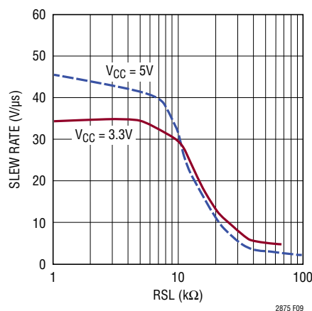
Figure 9. Slew Rate vs Slew Control Resistor RSL
