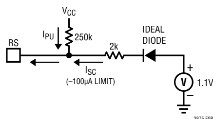
Figure 10. Equivalent Circuit of RS Pin
