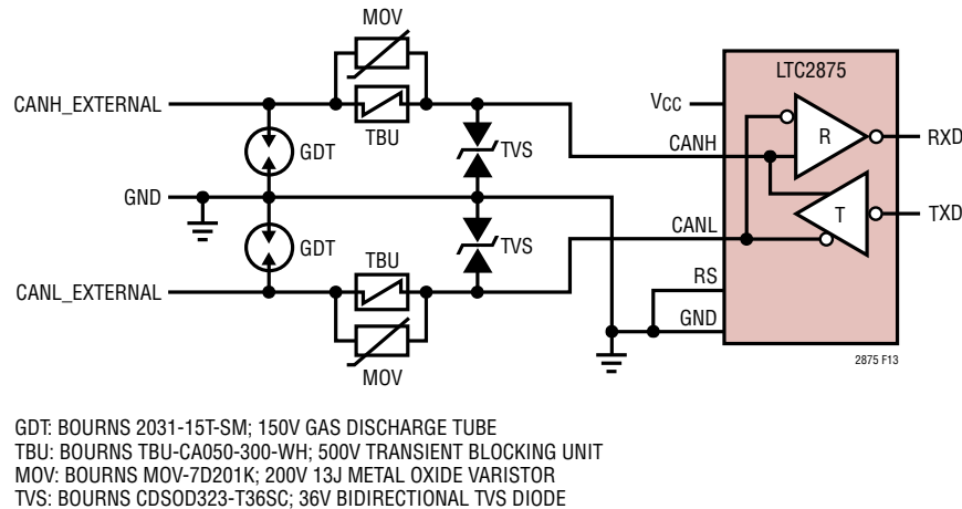
Figure 13. Network for IEC Level 4 Protection Against Surge, EFT and ESD
