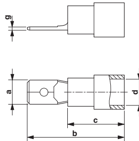
Dimensioned drawing
