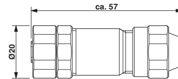
Dimensioned drawing
