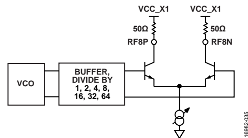
Figure 41. Output Stage
