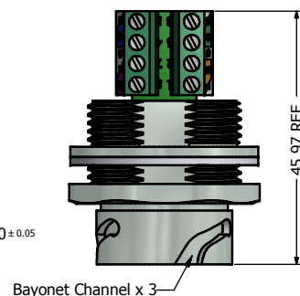
Bayonet Channel x 3
