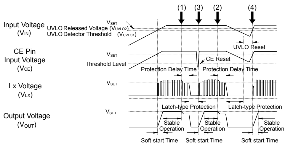
Timing Chart
