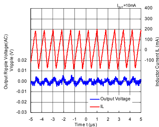
RP506Kxx1D/E/F V_{OUT} = 3.3\text{ V} ( V_{IN} = 5.0\text{ V} ) MODE = "H" Forced PWM Control
