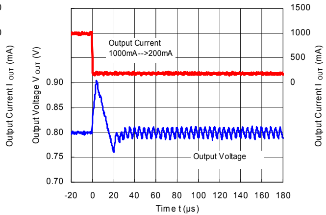
RP506Kxx1D/E/F ( V_{IN} = 3.6\text{ V} , V_{OUT} = 0.8\text{ V} ) MODE = "L" PWM/VFM Auto Switching Control
