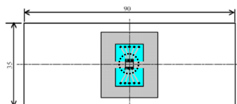
Highwattage Land Pattern
