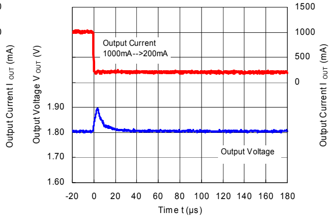
RP506Kxx1D/E/F ( V_{IN} = 3.6\text{ V} , V_{OUT} = 1.8\text{ V} )
