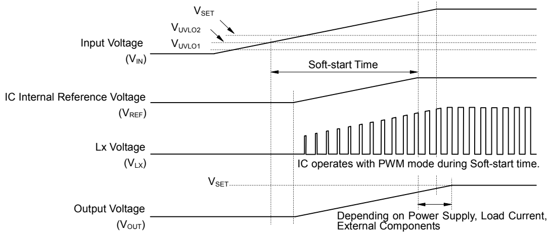
Timing Chart
