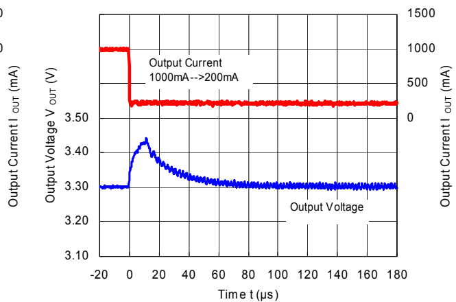
RP506Kxx1D/E/F ( V_{IN} = 5.0\text{ V} , V_{OUT} = 3.3\text{ V} ) MODE = "L" PWM/VFM Auto Switching Control
