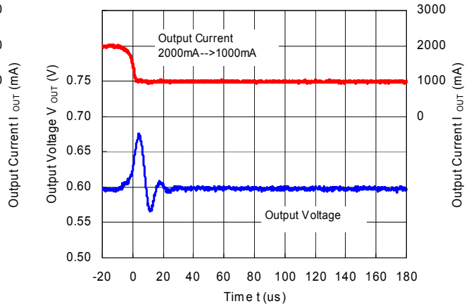
RP506Kxx1D/E/F ( V_{IN} = 3.6\text{ V} , V_{OUT} = 0.8\text{ V} ) MODE = "L" PWM/VFM Auto Switching Control
