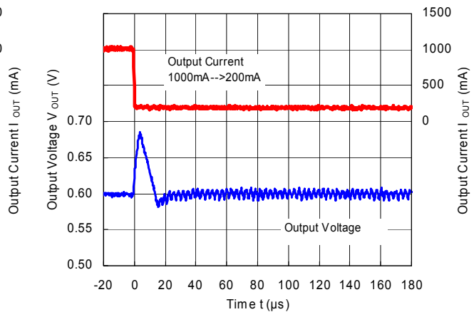
RP506Kxx1D/E/F ( V_{IN} = 3.6\text{ V} , V_{OUT} = 0.6\text{ V} ) MODE = "L" PWM/VFM Auto Switching Control
