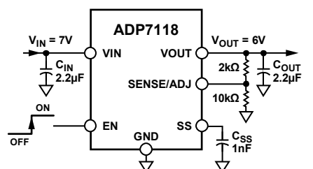
Figure 2. ADP7118 with 5 V Output Adjusted to 6 V
