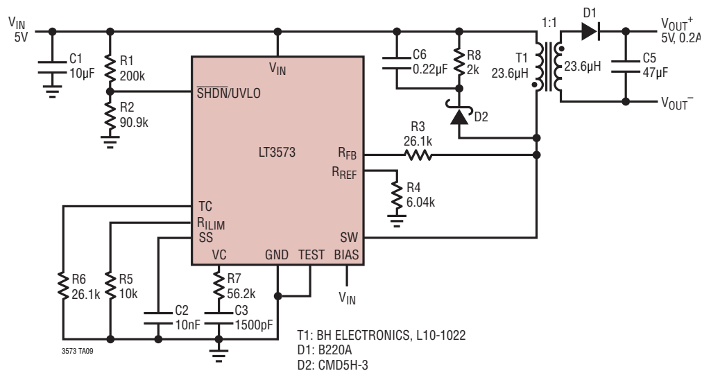
5V Isolated Flyback Converter Using Coupling Inductor
