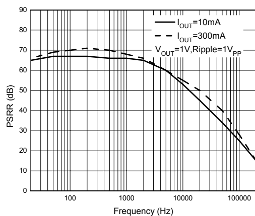
Figure 33. PSSR vs. Frequency (Conditions: C_{IN} = C_{OUT} = 1\mu\text{F} , V_{IN} = 2.5\text{V} , V_{OUT} = 1\text{V} \text{Ripple} = 1V_{PP} )
