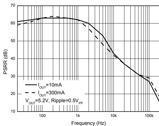
Figure 35. PSSR vs. Frequency (Conditions: C_{IN} = C_{OUT} = 1\mu\text{F} , V_{IN} = 6\text{V} , V_{OUT} = 5.2\text{V} \text{Ripple} = 0.5V_{PP} )
