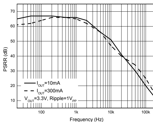
Figure 34. PSSR vs. Frequency (Conditions: C_{IN} = C_{OUT} = 1\mu\text{F} , V_{IN} = 4.3\text{V} , V_{OUT} = 3.3\text{V} \text{Ripple} = 1V_{PP} )
