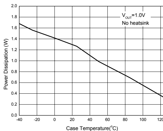
Figure 28. Power Dissipation vs. Case Temperature
