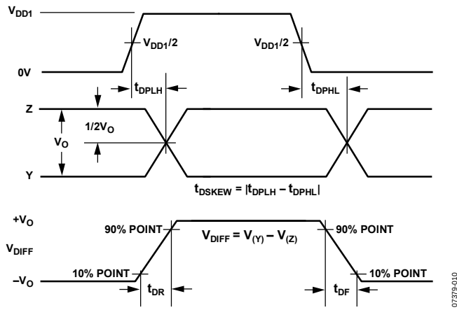
Figure 26. Driver Propagation Delay, Rise/Fall Timing
