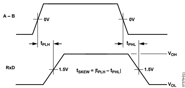
Figure 27. Receiver Propagation Delay
