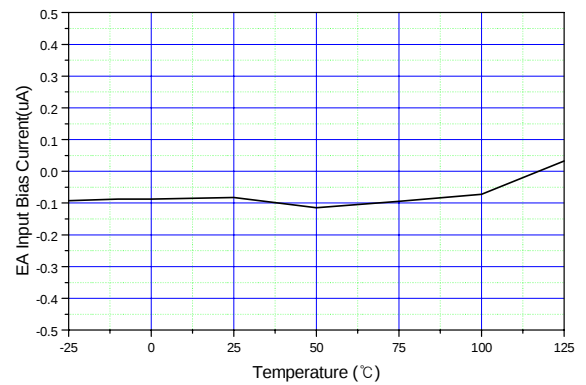
Figure 10. Error Amplifier Input Bias Current vs Temperature
