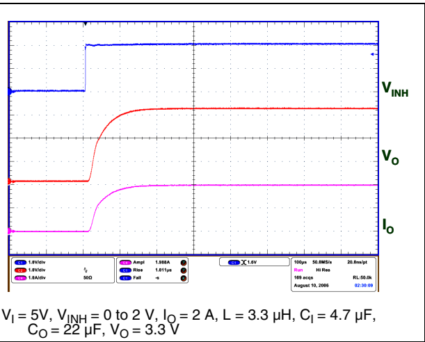
Figure 20. Inhibit transient
