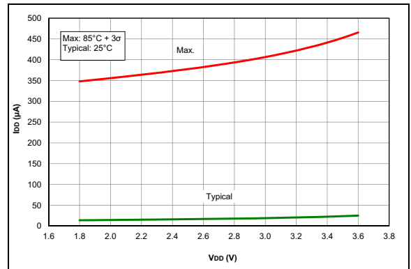
FIGURE 27-35: I_{PD} , ADC Non-Converting, PIC16LF1703/7 only
