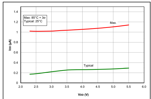
FIGURE 27-36: I_{PD} , ADC Non-Converting, PIC16F1703/7 only
