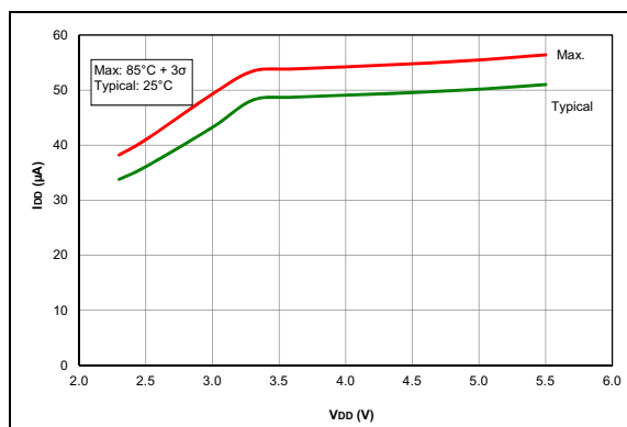
FIGURE 27-4: I_{DD} , EC Oscillator, Low-Power Mode, F_{OSC} = 500\text{ kHz} , PIC16LF1703/7 Only.
