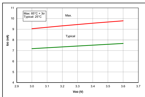
FIGURE 27-27: I_{DD} , Brown-Out Reset (BOR), BORV = 1 , PIC16LF1703/7 only.
