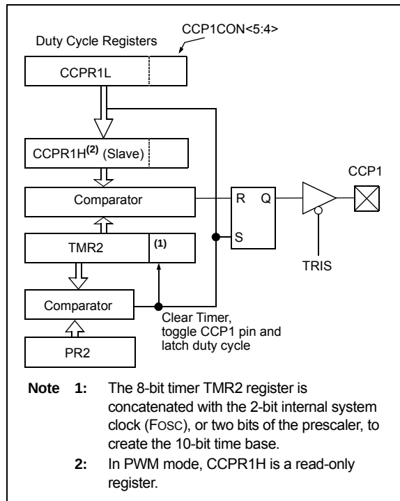
FIGURE 22-4: SIMPLIFIED PWM BLOCK DIAGRAM
