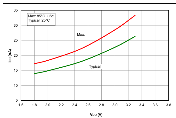
FIGURE 27-25: I_{DD} , Fixed Voltage Reference (FVR), PIC16LF1703/7 only.
