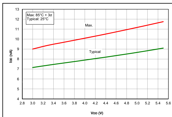
FIGURE 27-28: I_{DD} , Brown-Out Reset (BOR), BORV = 1 , PIC16F1703/7 only.
