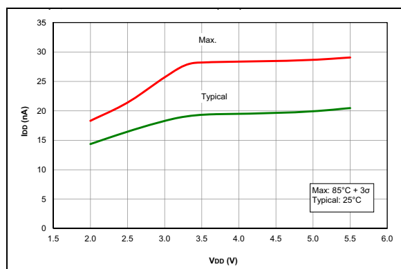
FIGURE 27-26: I_{DD} , Fixed Voltage Reference (FVR), PIC16F1703/7 only.
