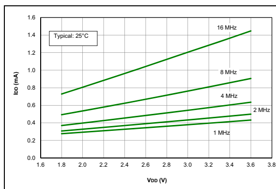
FIGURE 27-17: I_{DD} Typical, HFINTOSC Mode, PIC16LF1703/7 Only.
