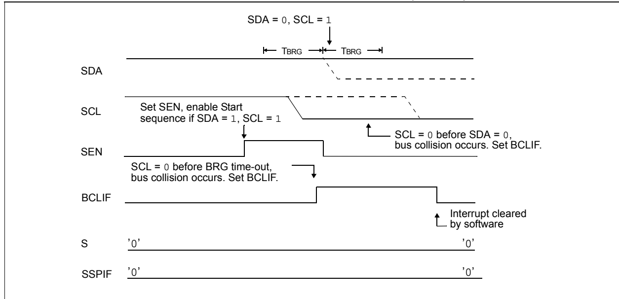
FIGURE 23-35: BRG RESET DUE TO SDA ARBITRATION DURING START CONDITION
