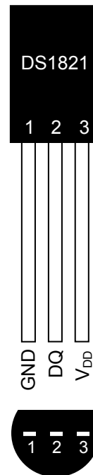
(BOTTOM VIEW)
