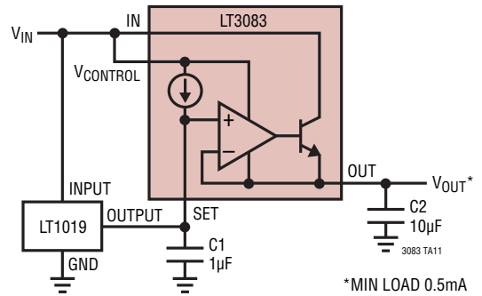
Reference Buffer
