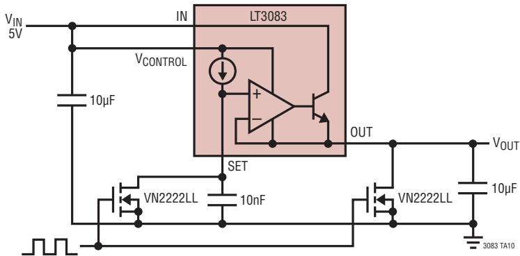
Ramp Generator
