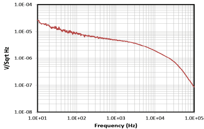
LDO2=1.8V Noise Spectral Density
