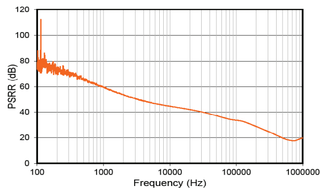
LDO2=1.8V, PSRR, Iout=100mA
