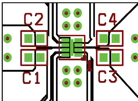
Figure 3 — SC563 Layout Example
