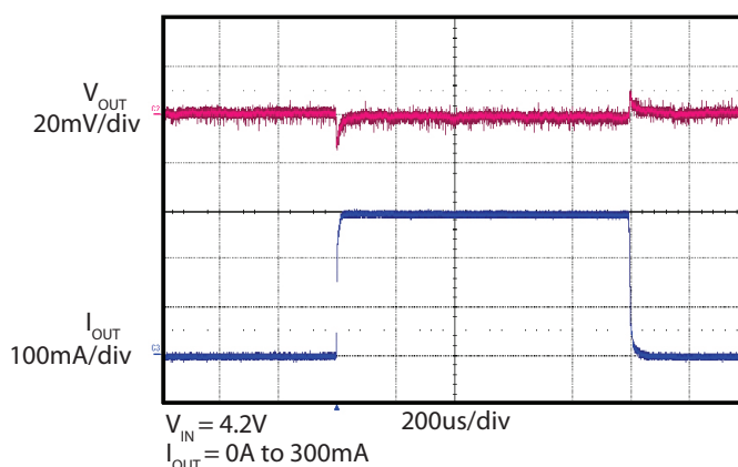
LDO2=1.8V, 0 to 300mA Load Transient
