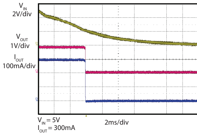
Shutdown ( V_{OUT}=1.8V )
