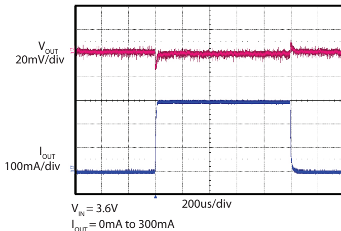
LDO2=1.8V, 0 to 300mA Load Transient
