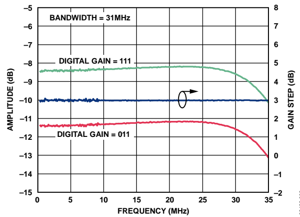
Figure 9. Gain Step and Gain Error vs. Frequency (Bandwidth Setting = 31 MHz, V_{\text{GAIN}} = 0\text{ V} )
