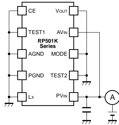
Standby Current
