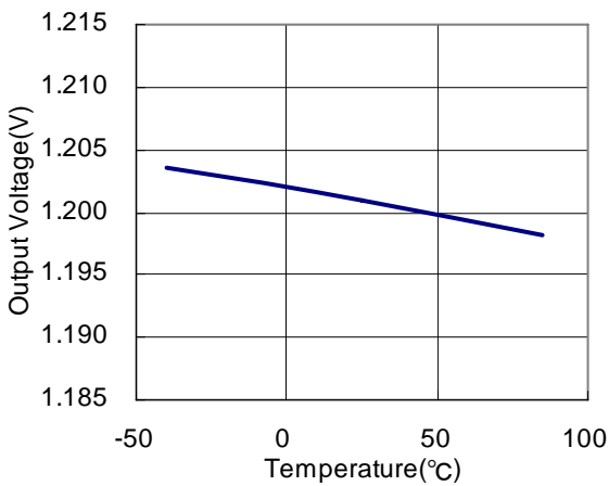
RP501K121x(PWM fixed) V IN =3.6V, MODE=0V, I OUT =500mA
