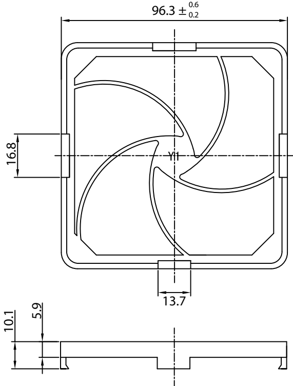
RETAINER
