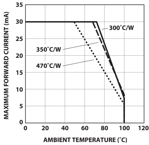
Figure 7: Maximum Forward Current vs. Ambient Temperature, Derated Based on T_{jmax} = 110^{\circ}C (InGaN)
