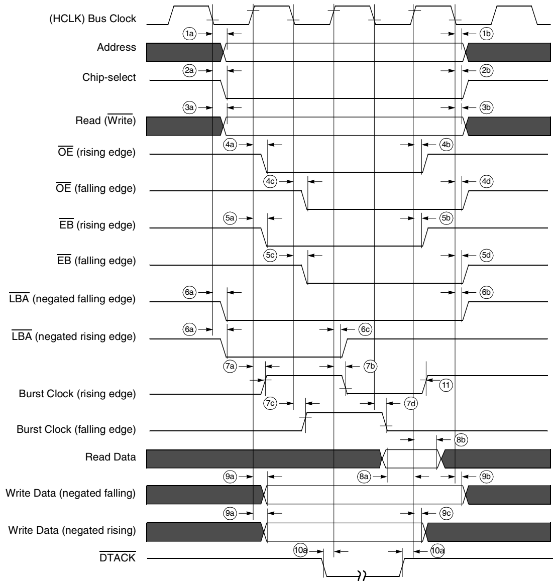
Figure 45. EIM Bus Timing Diagram
