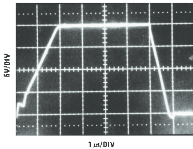
Figure 41. LF356
