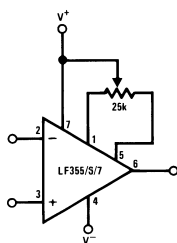
Figure 36. V_{OS} Adjustment
