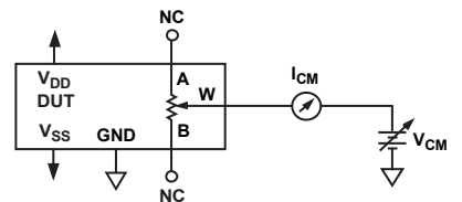
Figure 30. Common-Mode Leakage Current
